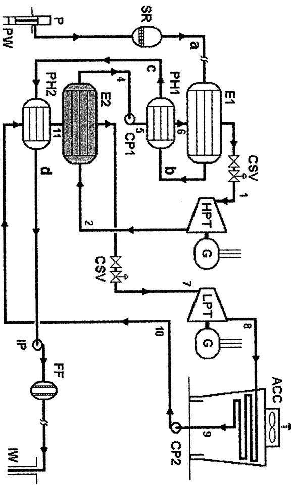
Fig. 8.13 Dual-fluid cascaded binary cycle featuring a heat recuperator.
